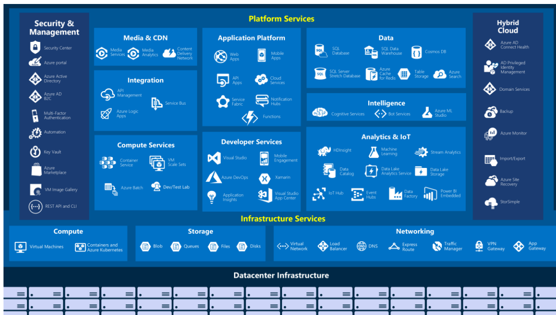
Azure Services
