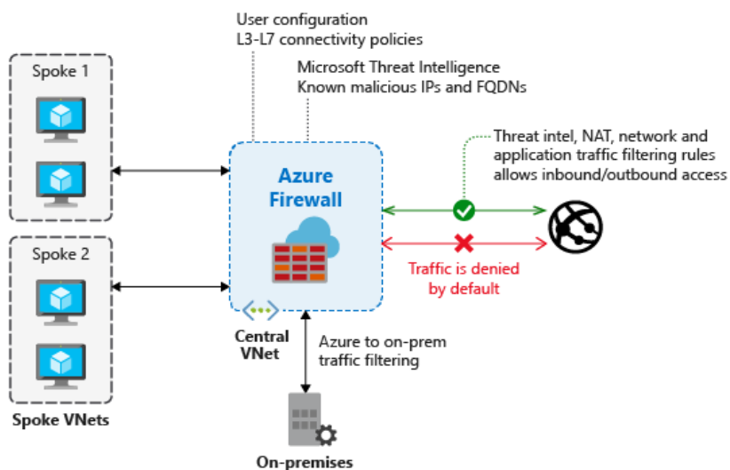
Azure Firewall
